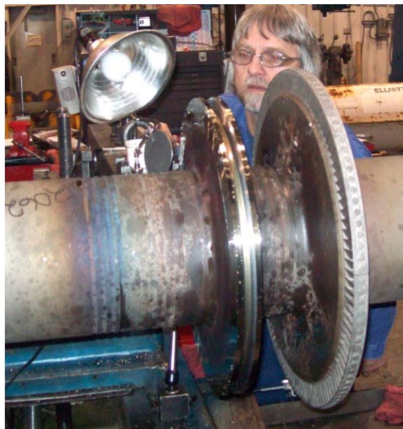
Machined turbine disk ready for reblading
