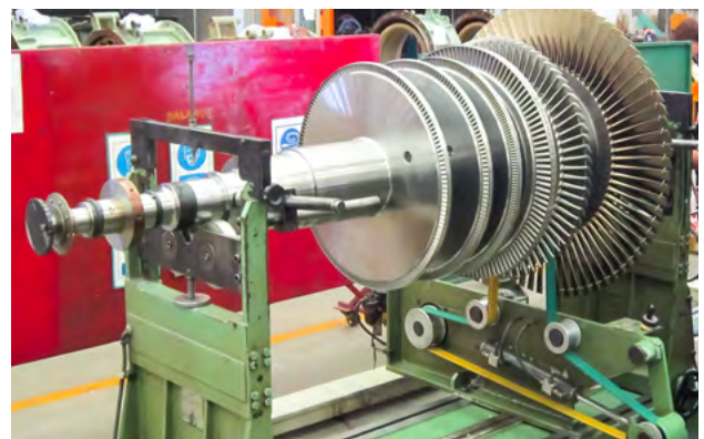
AMC dynamic balancing equipment.
