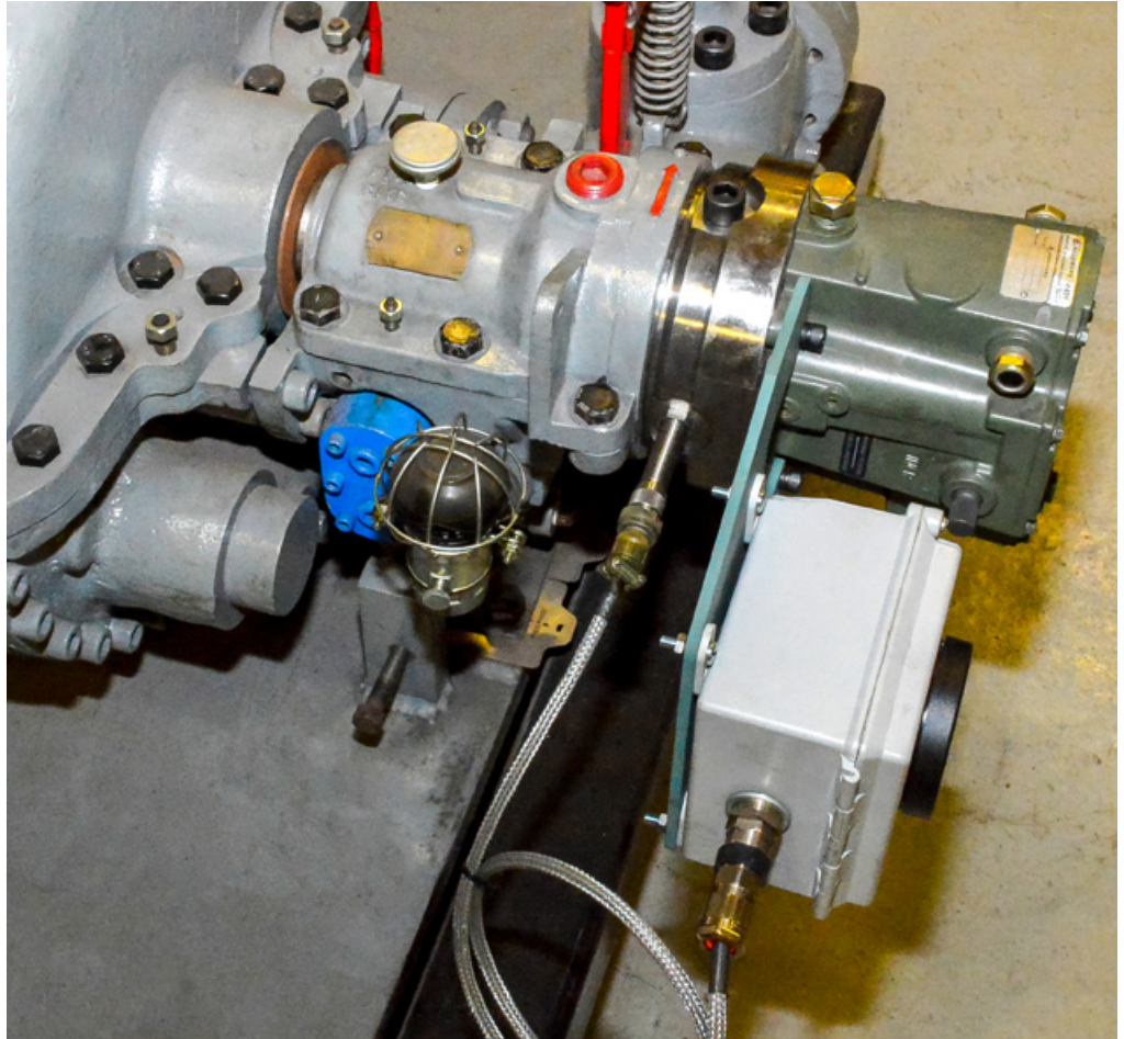
Installed TG Governor Tachometer Kit showing connection to governor.
