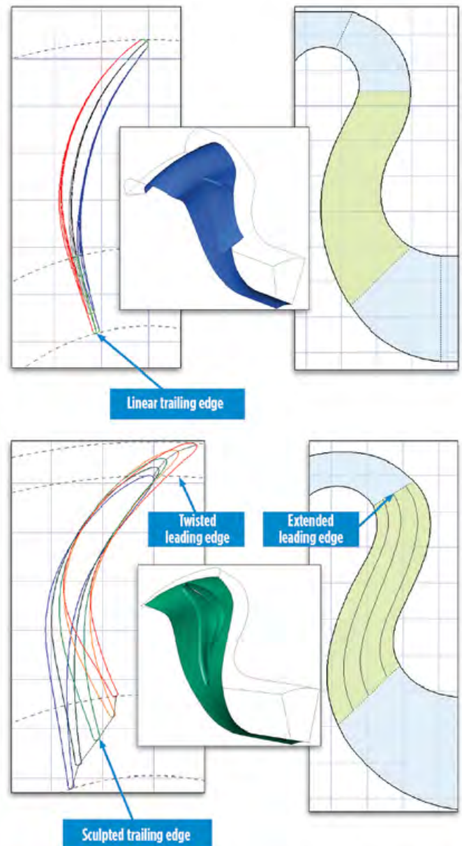
FIG. 5. Return channel vane design iterations. Generation 1 (top) has a 2D return channel, while Generation 2 (bottom) has a 3D return channel vane.
