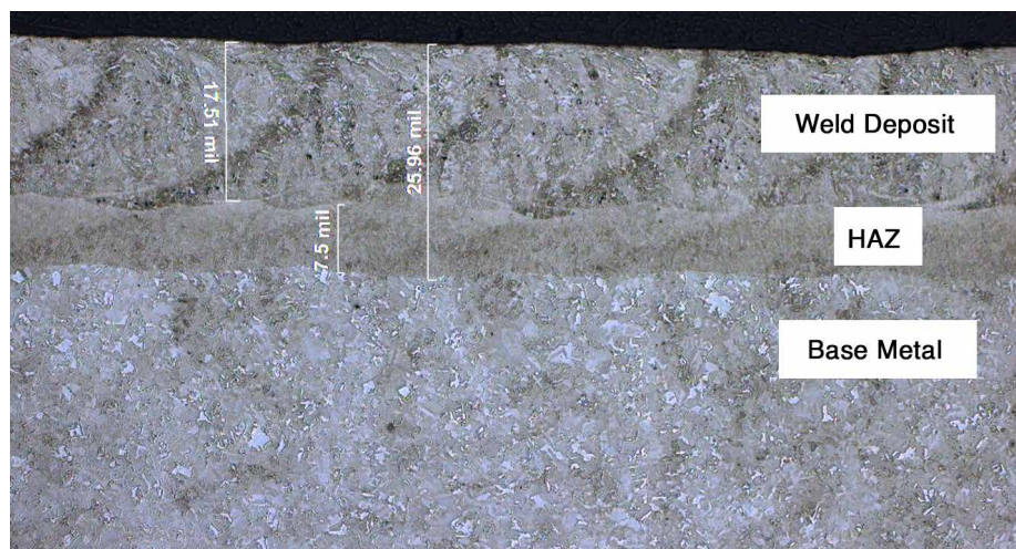
FIGURE 5 Cross Section of an LBW Overlay
